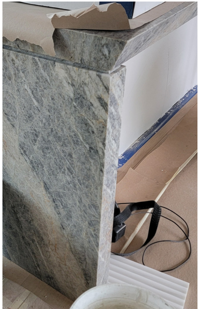
ANGLED MITERED EDGE WITH STONE REGLET DETAIL
